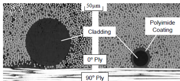
Fig.1. Standard SMF (left) and thin optical fiber cross-section embedded in a CFRP lamina [1].
