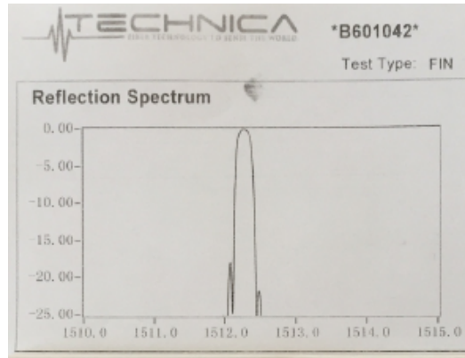
Fig.5. Typical thin FBG reflection spectrum with high side lobe suppression.
